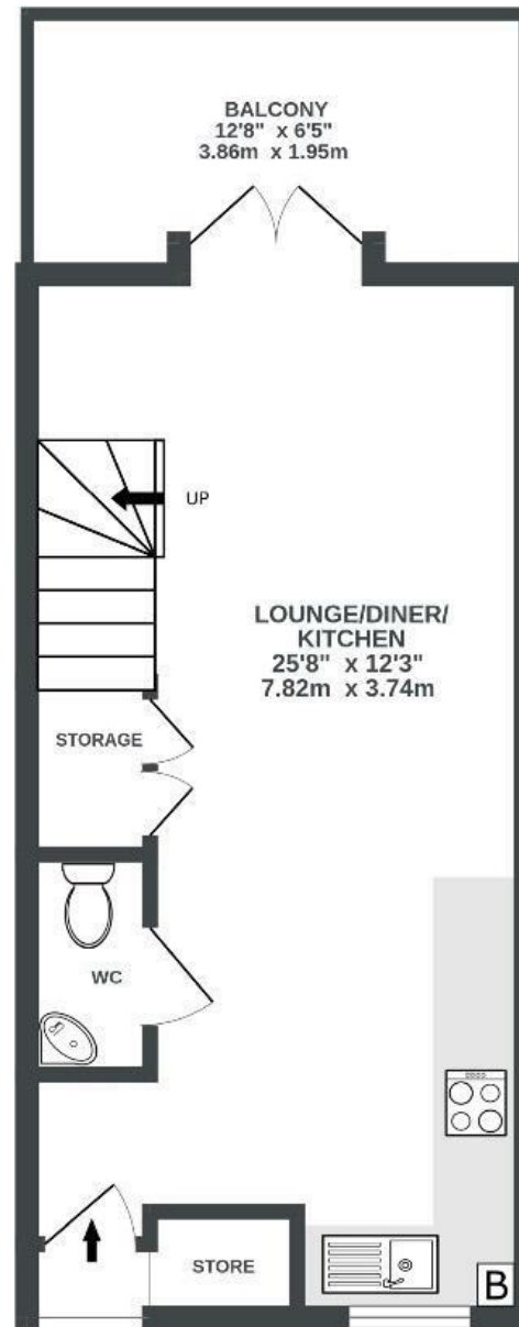
GROUND FLOOR 318 sq.ft. (29.6 sq.m.) approx.
